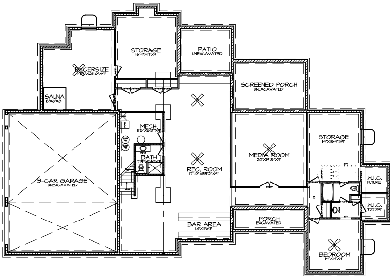
FOUNDATION PLAN A-2
