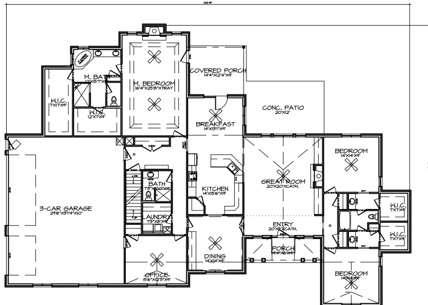
FIRST FLOOR PLAN A-3
